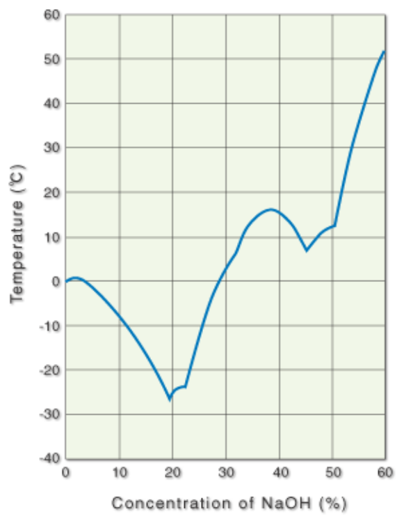
■ Freezing Point Curve of Caustic Soda Solution
